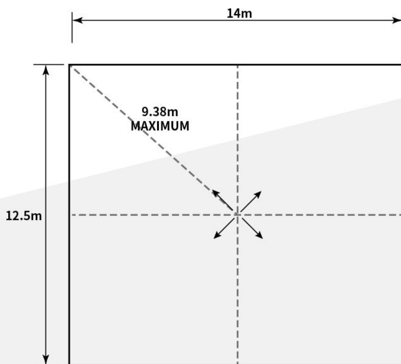
360° Radial Nozzle (8 Port) Arrangement
