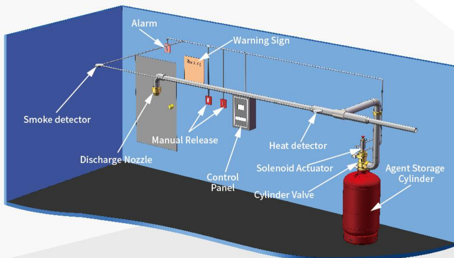
Typical Clean Agent System Layout
