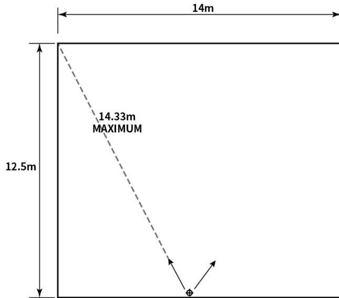
180° Sidewall Nozzle (8 Port) Arrangement
